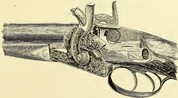
Mr. J. Walsh's Pin-fire Gun.
